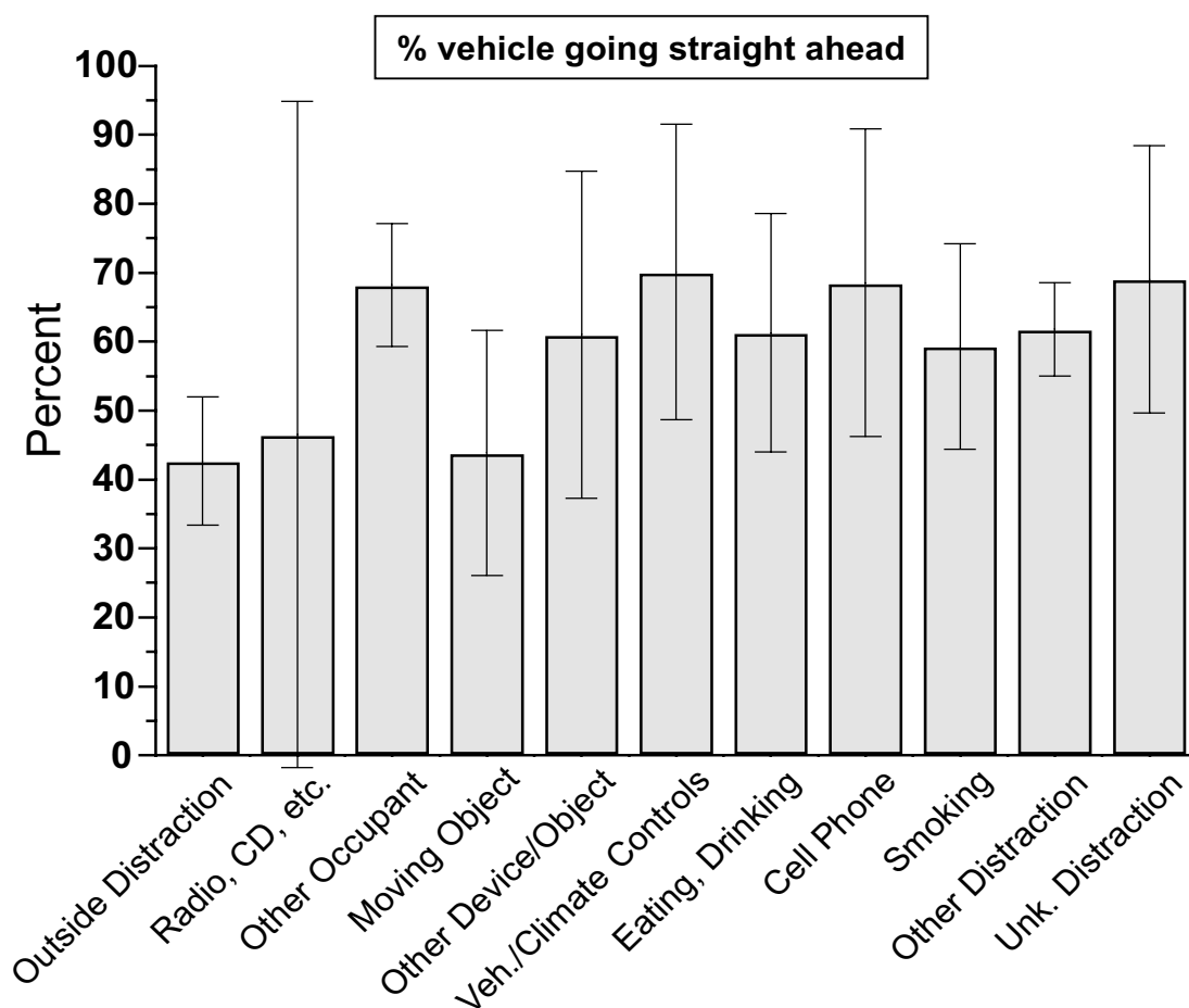
Figure B.20. Effect of precrash vehicle maneuver on specific driver distraction.
