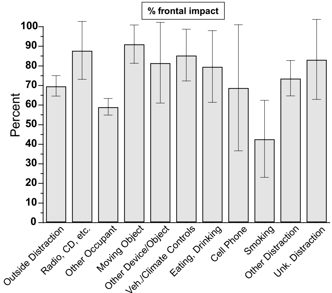
Figure B.22. Effect of region of impact on specific driver distraction.
