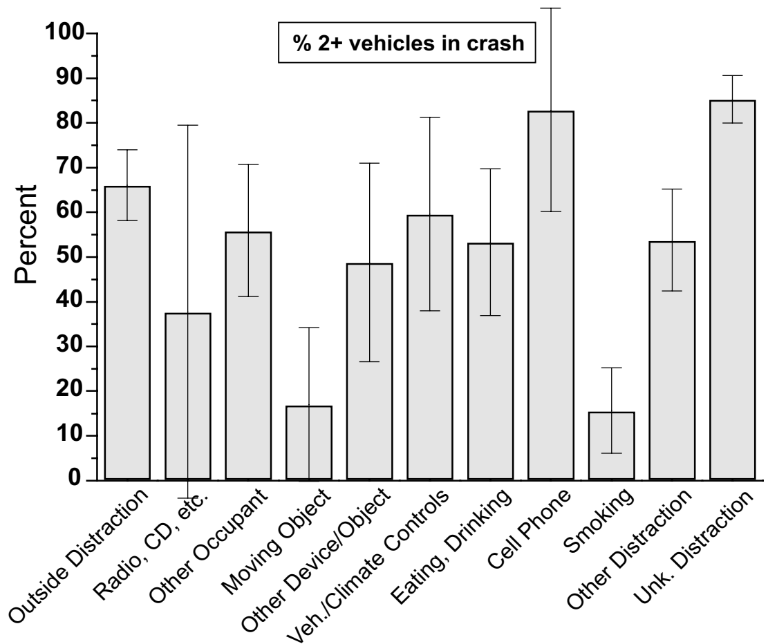
Figure B.18. Effect of number of vehicles on specific driver distraction.
