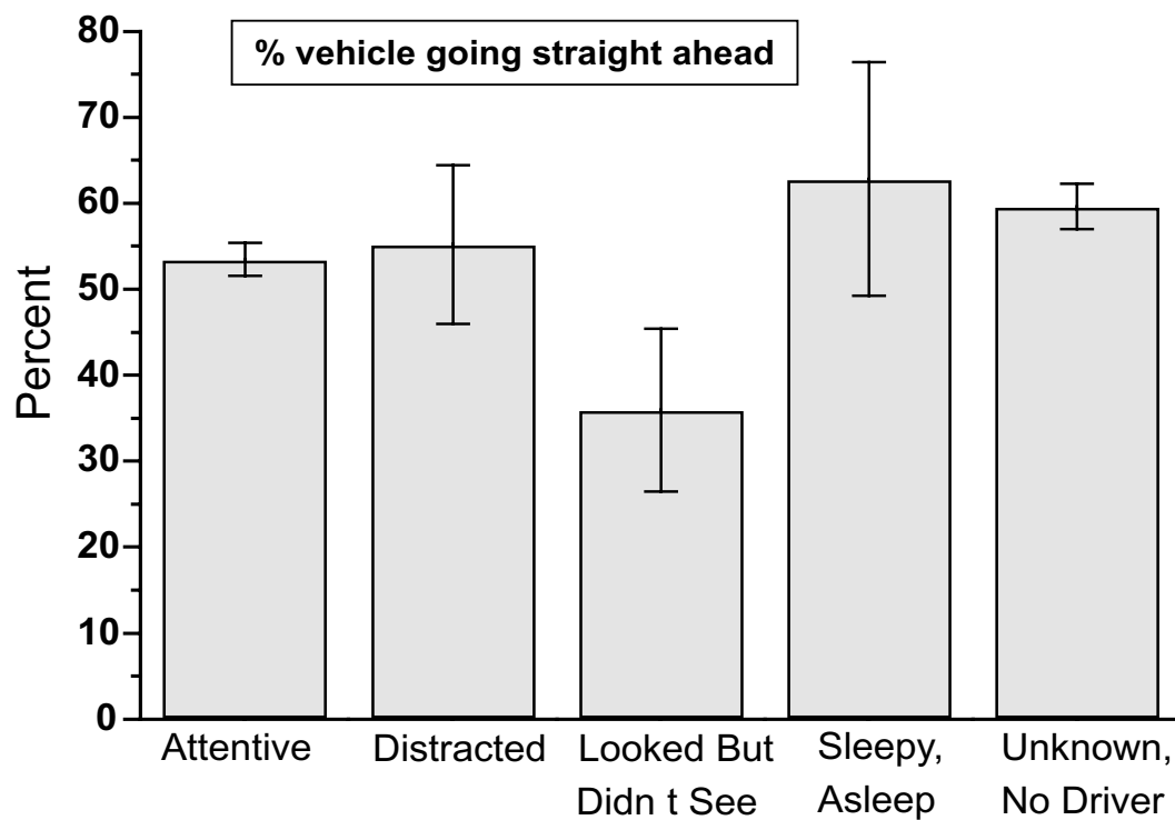
Figure B.19. Effect of precrash vehicle maneuver on driver attention status.
